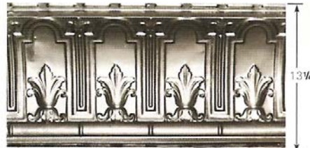
No. 807 CORNICE 9 1/2" Projection 9 1/2" Deep 48" Long
